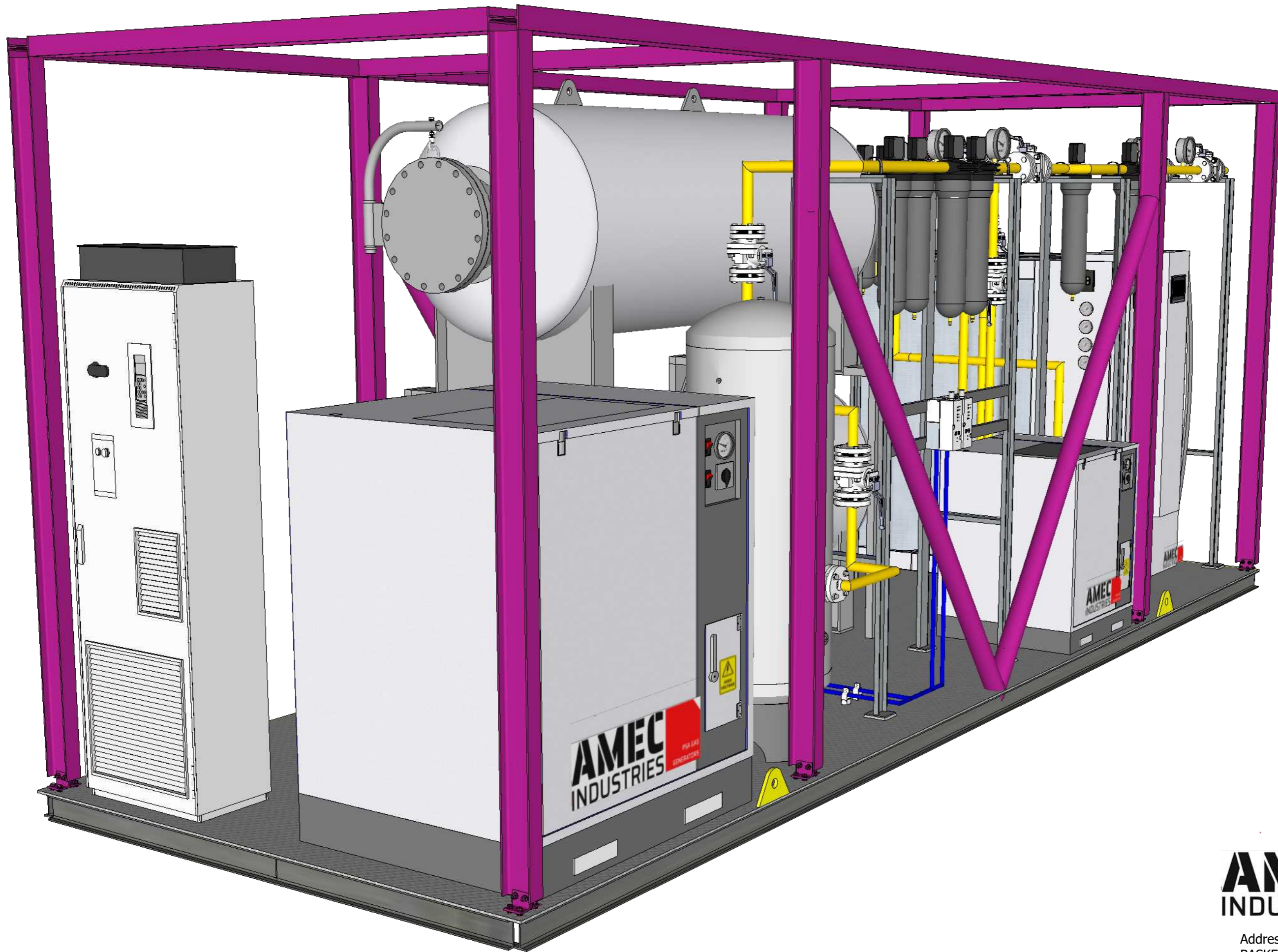
SKID MOUNTED OXYGEN GENERATION PLANT
